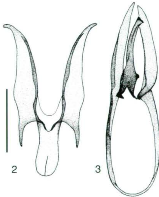
Fig. 1: Hydrocyphon gereckei sp.n., habitus. Scale bar, 1 mm. Fig. 2-3: Hydrocyphon gereckei sp.n. 2 – tegmen, dorsal view; 3 – aedeagus, dorsal view. Scale bar, 0,25 mm.
